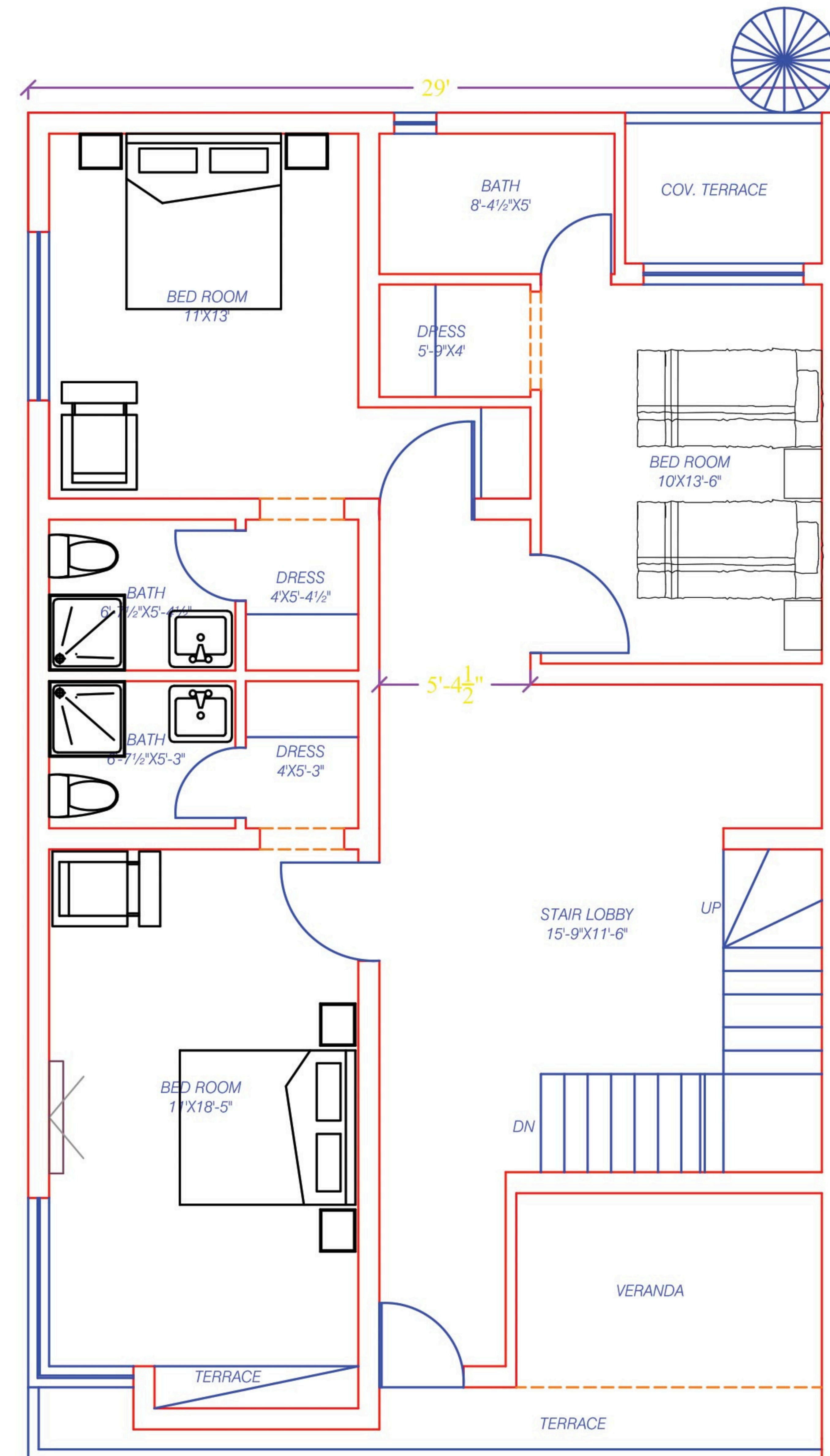
FIRST FLOOR PLAN COVERED AREA = 1333.00 Sft.
