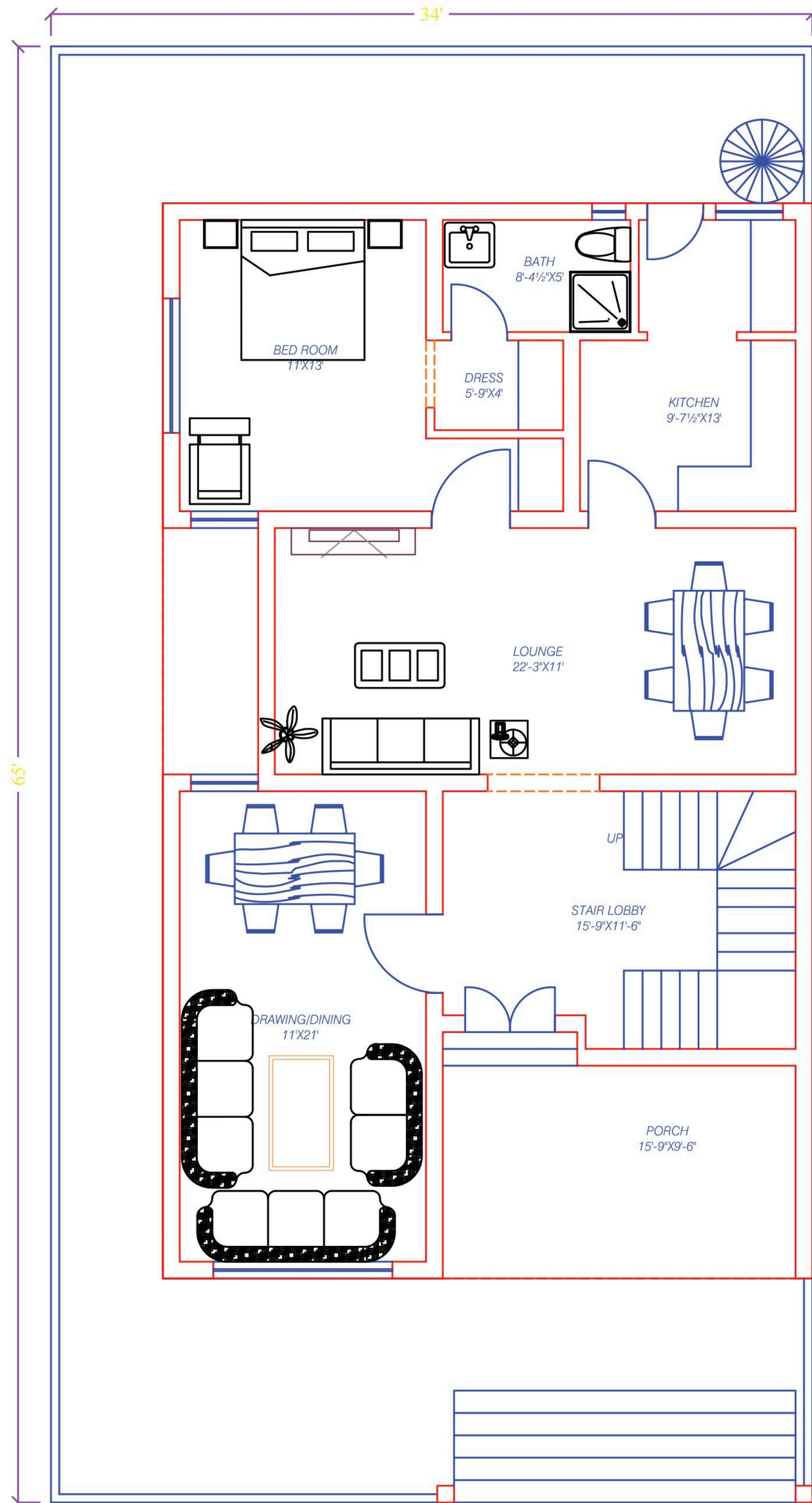
GROUND FLOOR PLAN COVERED AREA = 1392.00 Sft.
