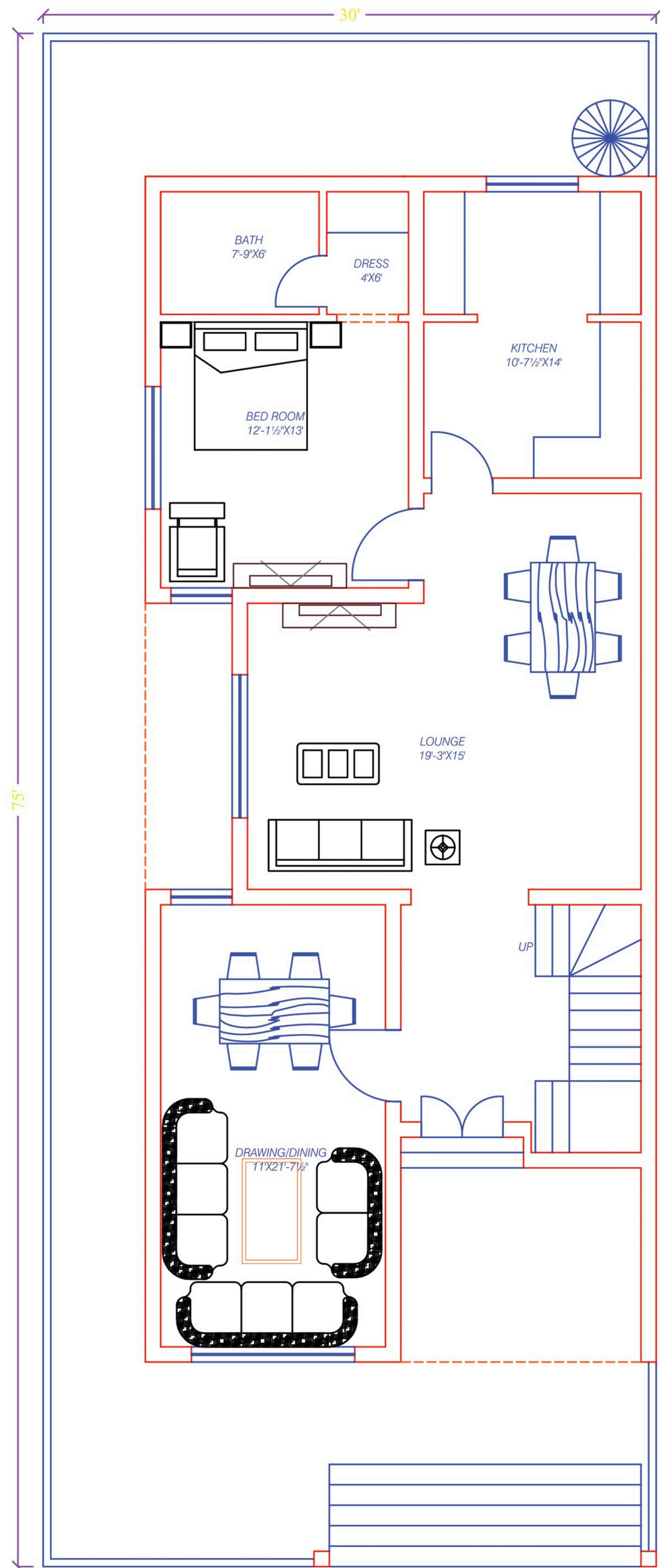
GROUND FLOOR PLAN COVERED AREA = 1450.00 Sft.
