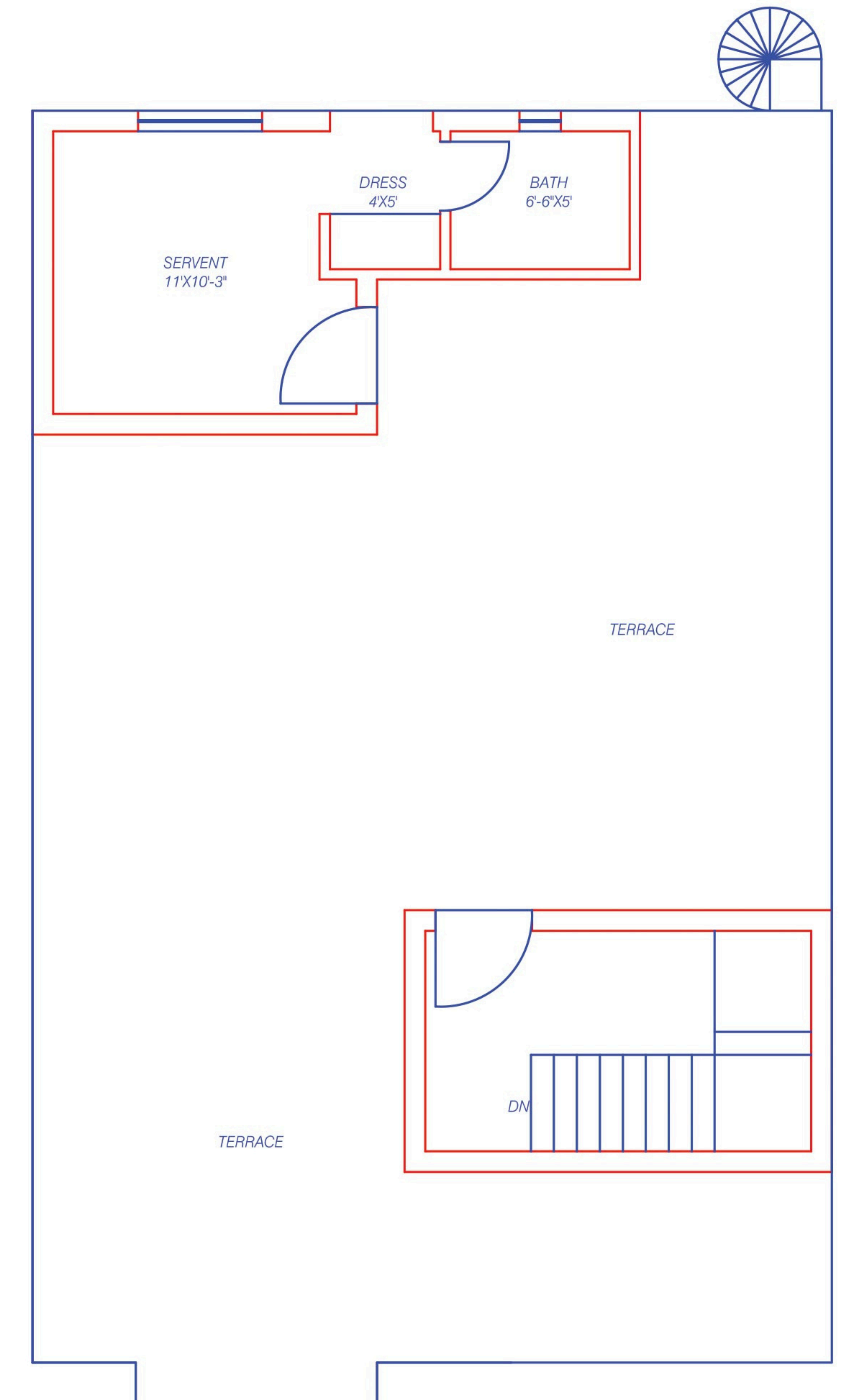
MUMTY FLOOR PLAN COVERED AREA = 352.00 Sft. TOTAL COVERED AREA = 3077.00 Sft.
