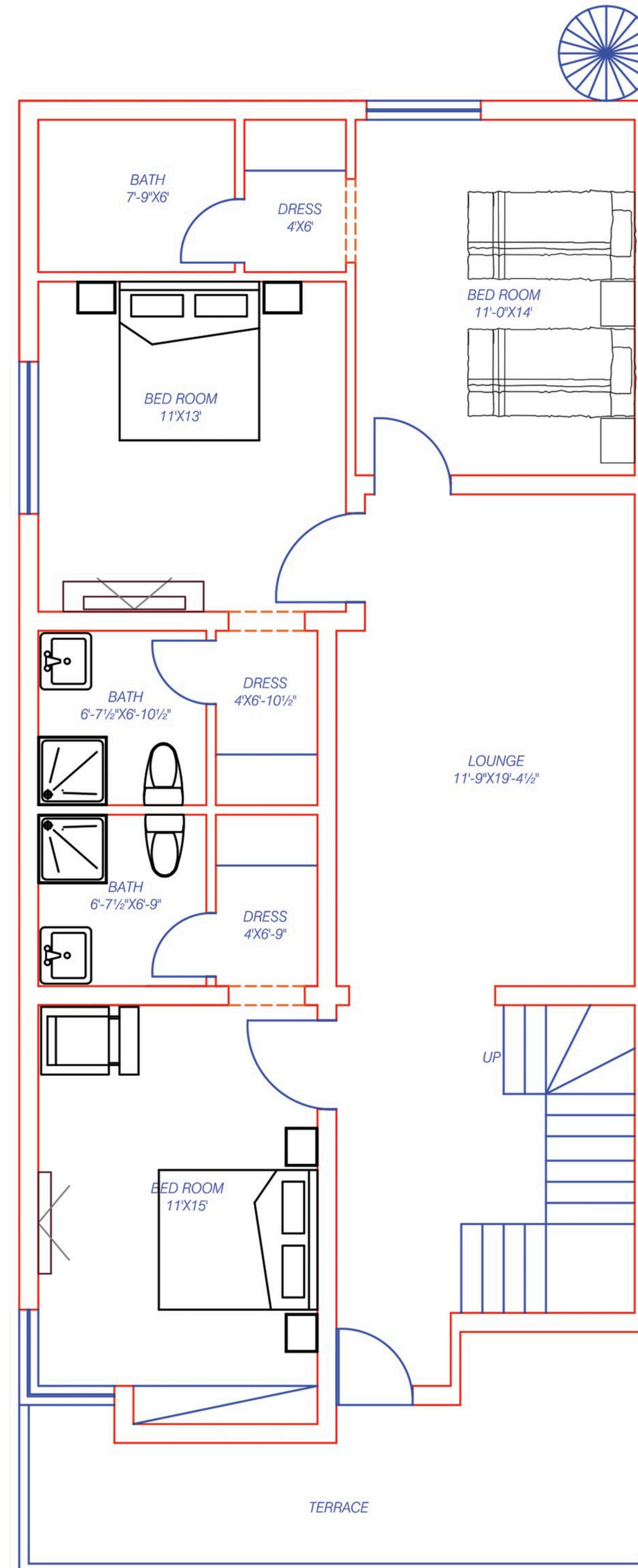
FIRST FLOOR PLAN COVERED AREA = 1275.00 Sft.
